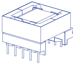
EFD 25 reinforced insulation creepage distances: 6mm
