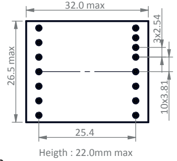
EF 25 reinforced insulation creepage distances: 8mm
