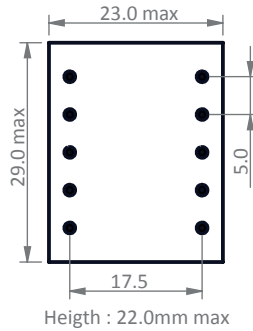
EI 28 reinforced insulation creepage distances: 6mm
