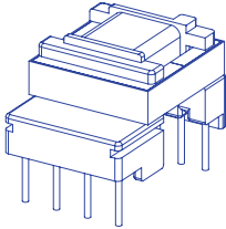
EF 12.6 reinforced insulation creepage distances: 6mm
