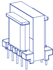
EF 25 reinforced insulation creepage distances: 6mm
