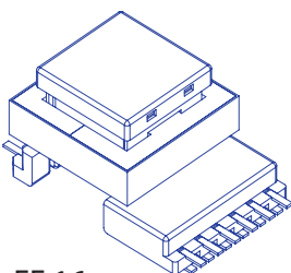
EF 16 reinforced insulation creepage distances: 6mm
