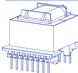
EF 20/11 reinforced insulation creepage distances: 6mm
