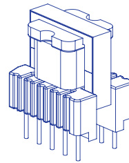
E 19 reinforced insulation creepage distances: 6mm
