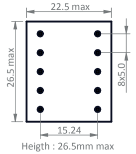
E 25 reinforced insulation creepage distances: 8mm
