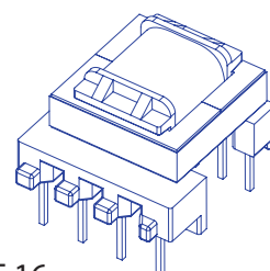
EF 16 reinforced insulation creepage distances: 6mm
