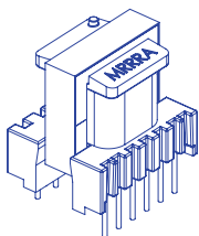
E 16 reinforced insulation creepage distances: 6mm
