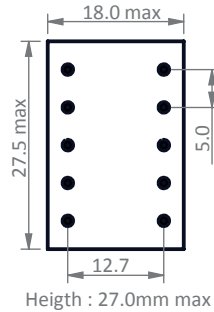
EF 25 reinforced insulation creepage distances: 6mm
