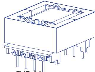
EVD 30 reinforced insulation creepage distances: 6mm
