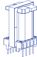
EL 19 reinforced insulation creepage distances: 6mm
