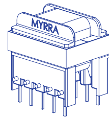
E 25 reinforced insulation creepage distances: 8mm
