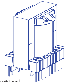
ETD Vertical reinforced insulation creepage distances: 6mm
