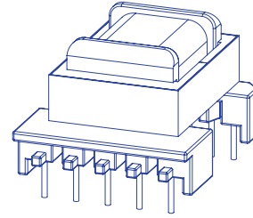
EF 25 reinforced insulation creepage distances: 6mm
