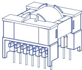
ETD Horizontal reinforced insulation creepage distances: 6mm
