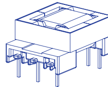
EFD 15 reinforced insulation creepage distances: 6mm
