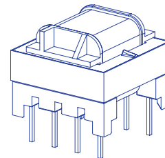
EF 20 basic insulation
