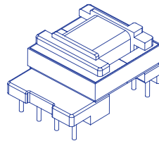
EF 12.6 reinforced insulation creepage distances: 6mm
