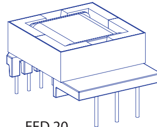
EFD 20 reinforced insulation creepage distances: 6mm
