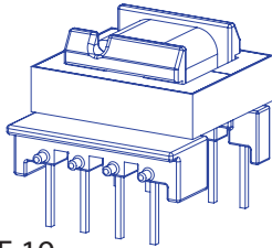
E 19 reinforced insulation creepage distances: 6mm
