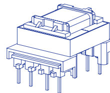
EF 16 reinforced insulation creepage distances: 6mm
