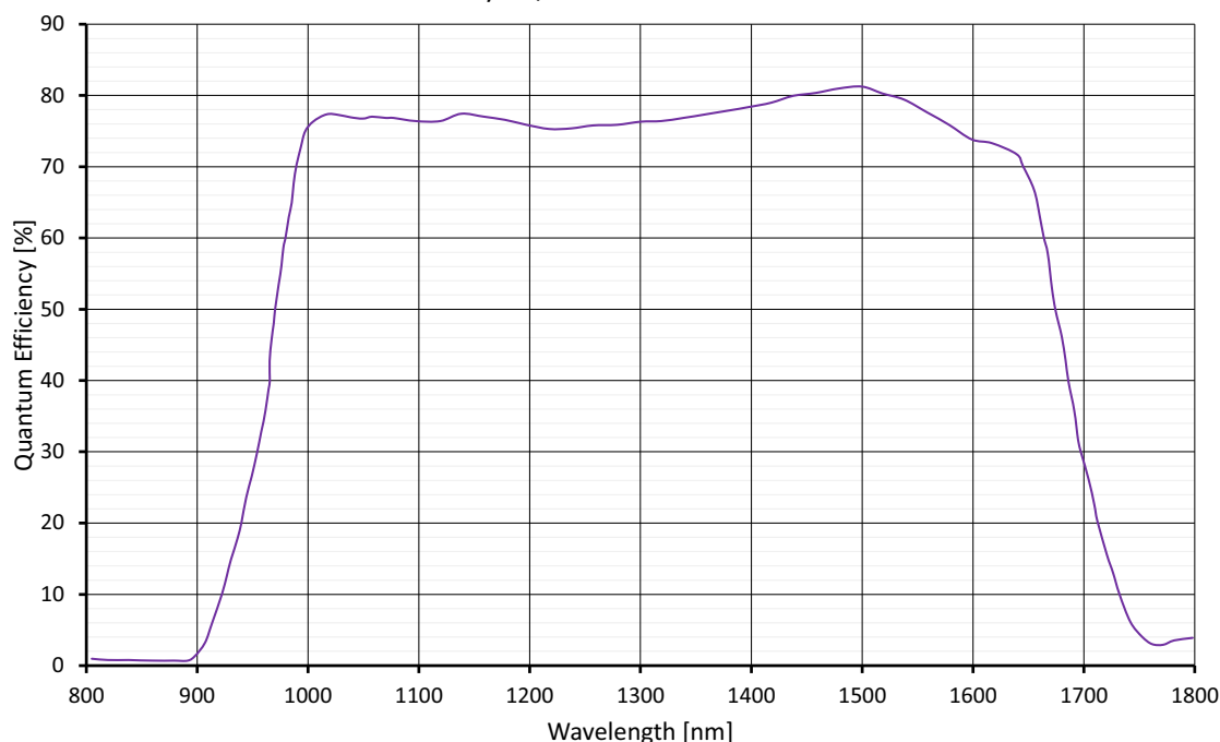
Figure 10: Goldeye G-033 SWIR TEC1 absolute QE
