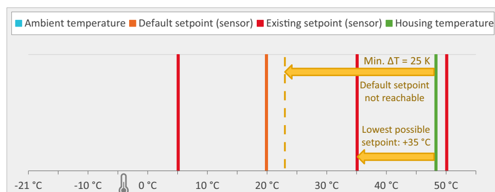
Figure 103: Cooling capabilities of Goldeye TEC1 models (example)
