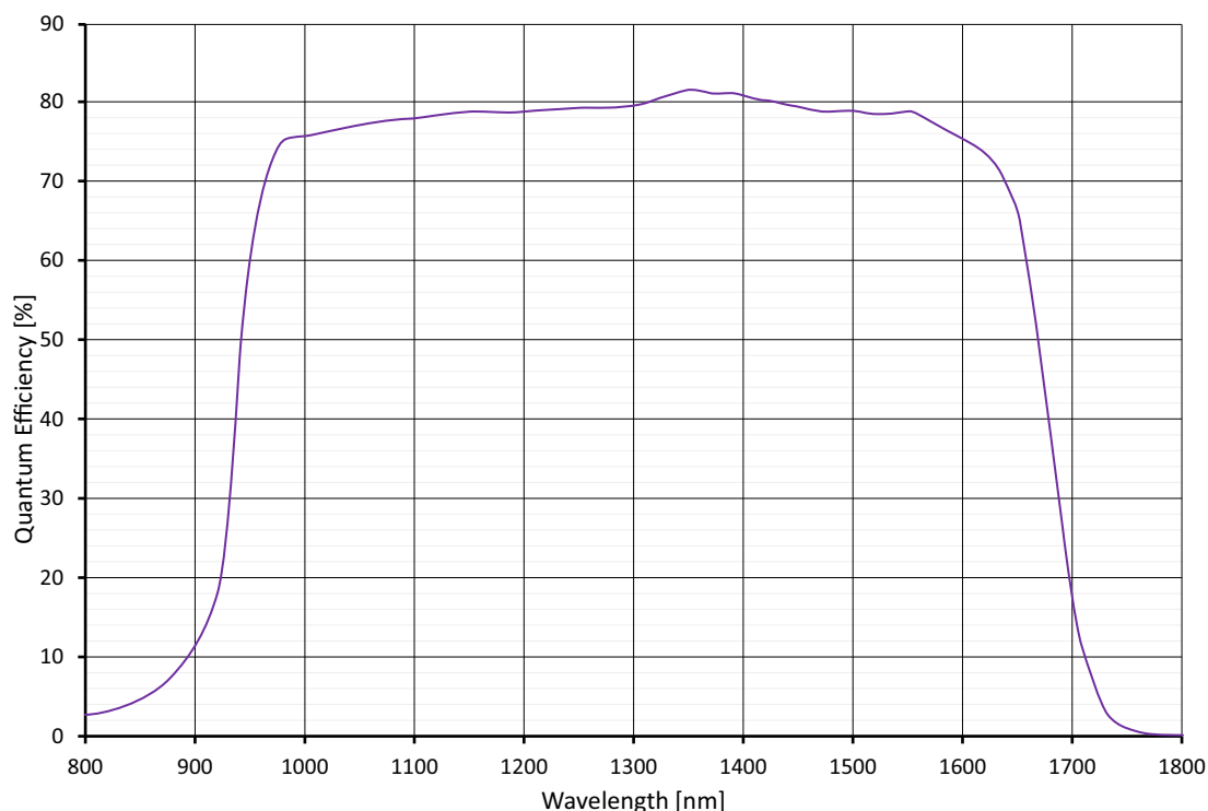
Figure 18: Goldeye CL-008 SWIR Cool TEC1 absolute QE
