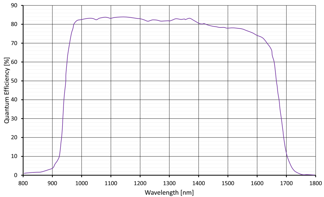
Figure 26: Goldeye CL-034 SWIR TEC1 absolute QE
