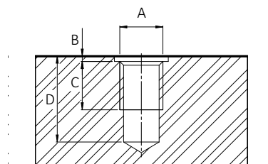
Figure 63: Front mounting threads for all Goldeye models
