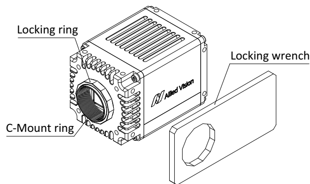
Figure 76: Goldeye camera with C-Mount adapter Type 2 and locking wrench
