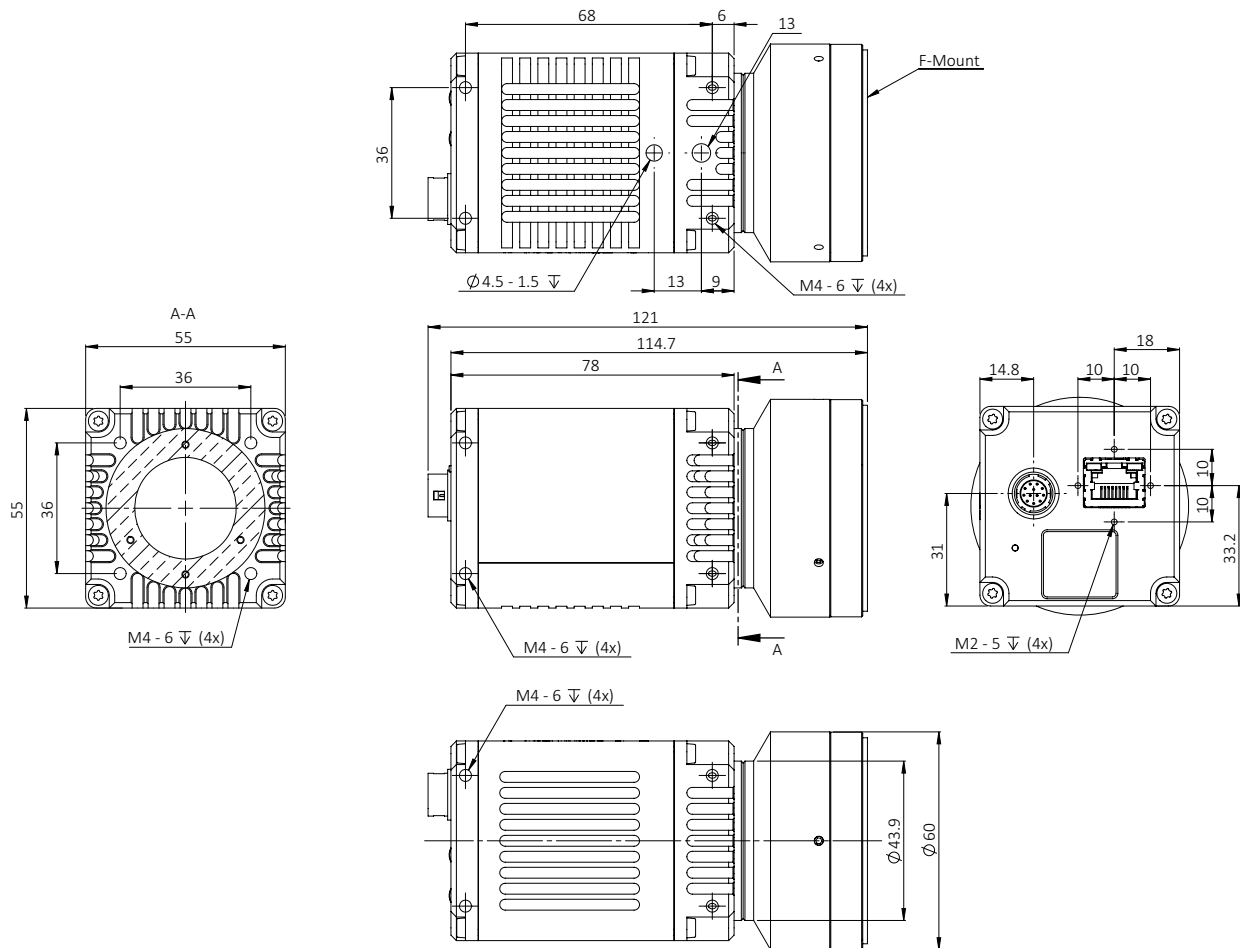
Figure 37: Goldeye G-034 SWIR TEC1 with F-Mount adapter
