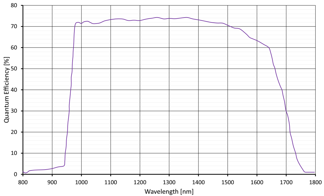
Figure 8: Goldeye G-032 SWIR TEC1 absolute QE
