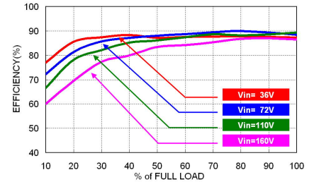
RHM20-110S05W Efficiency vs. Output Load
