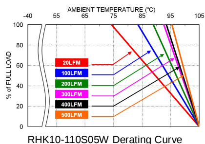
RHK10-110S05W Derating Curve
