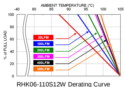
RHK06-110S12W Derating Curve
