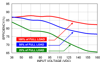
RHK06-110S12W Efficiency vs. Input Voltage
