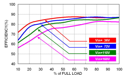
RHK06-110S12W Efficiency vs. Output Load
