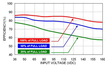
RHK03-110S24W Efficiency vs. Input Voltage
