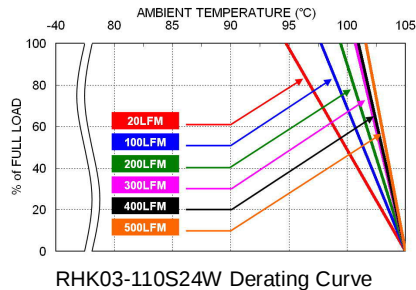
RHK03-110S24W Derating Curve
