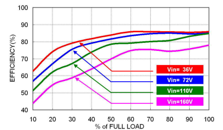
RHK03-110S24W Efficiency vs. Output Load
