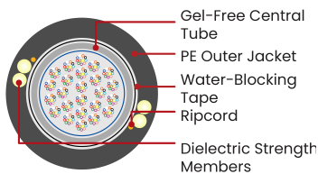
Dielectric Cable Cross-Section (features 4 strength rods)
