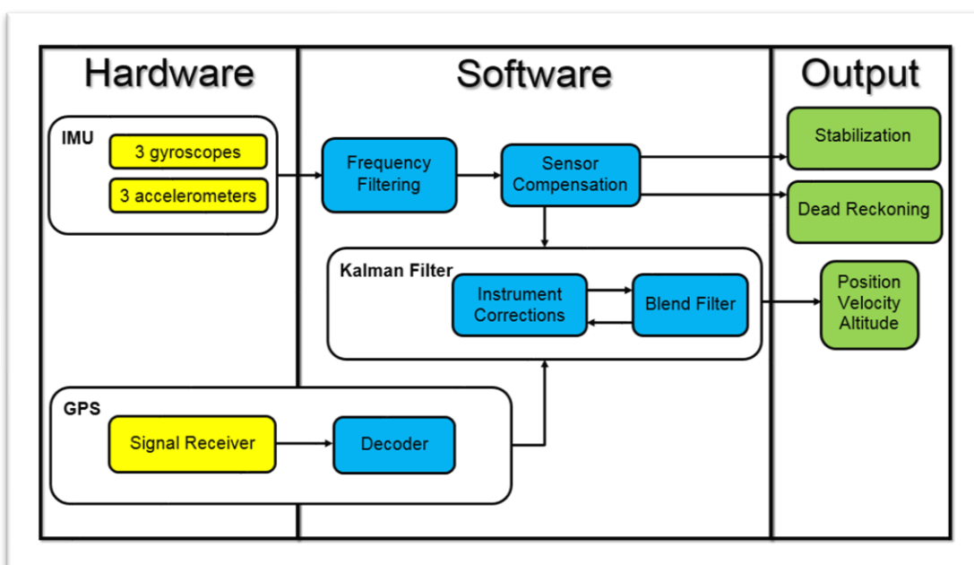
Figure 2: A possible configuration of INS in (S)UAVs
