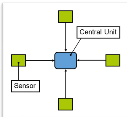
Figure 3: Server - Client
