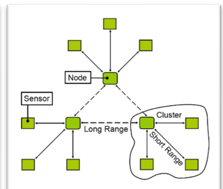
Figure 5: Two-tier
