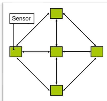
Figure 4: Peer-to-peer
