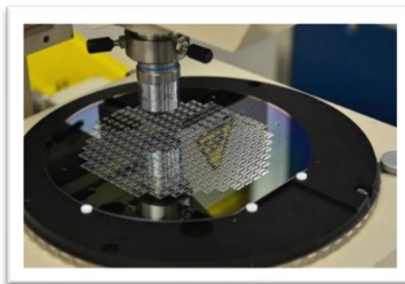
Figure 3: The inspection of the MEMS on a wafer
