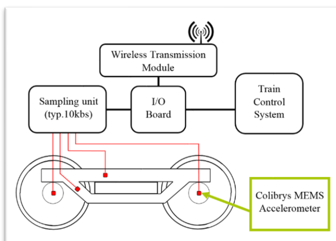
Figure 2: An example of bogie monitoring configuration
