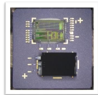
Figure 2: A VC Sensor from Safran Top: ASIC. Bottom: MEMS die
