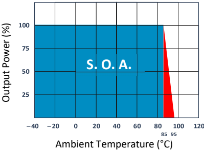
Only 24 Vdc Input Models
