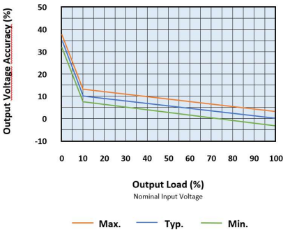
All Other Models
