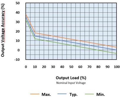
Only 3.3 Vdc Input Models and following: RS4-0515D10AX RS4-0503S10AX / RS4-0503D10AX RS4-0505S10AX / RS4-0505D10AX
