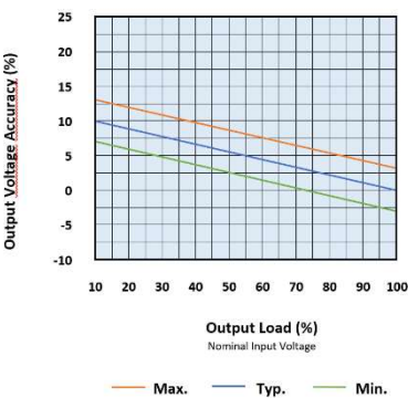
Output Voltage Tolerance
