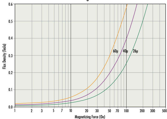
DC Magnetization
