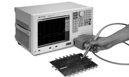
E4990A-120 with 42941A
