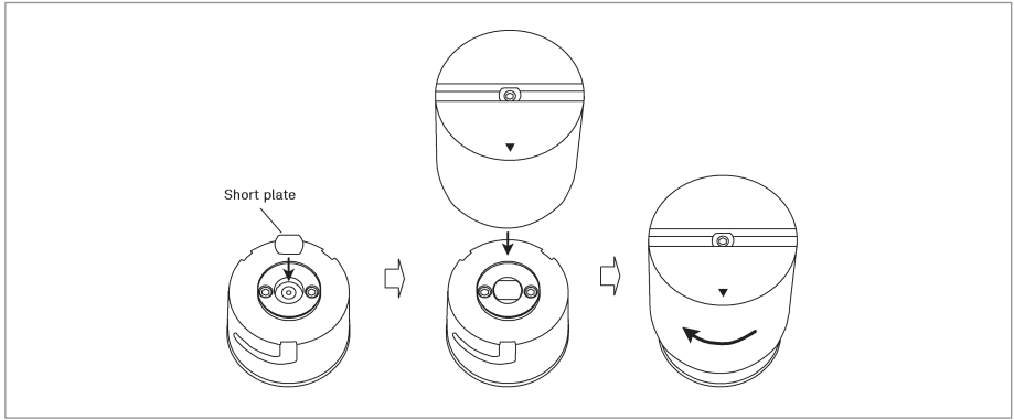
Short compensation
