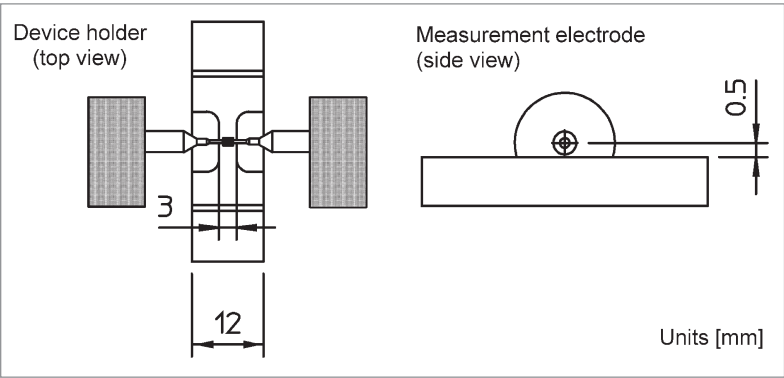
Electrode dimensions
