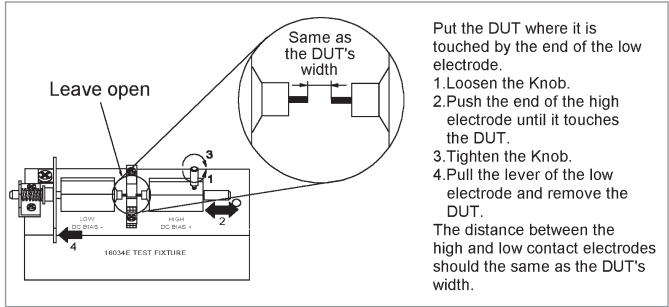
Open compensation
