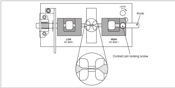
Short compensation
