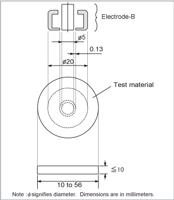
Material size for electrode-B
