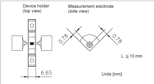
Electrode dimensions
