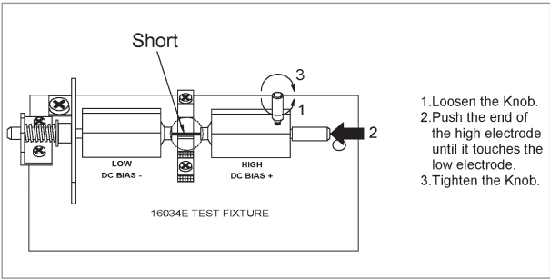
Short compensation
