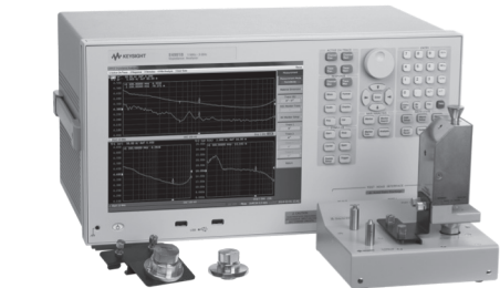
E4991B with 16453A
