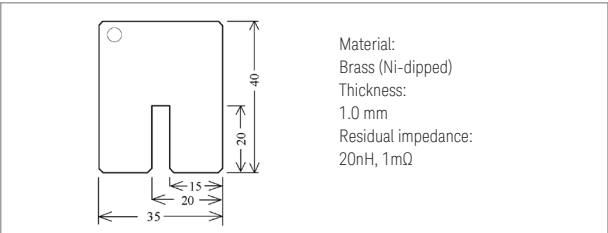
Shorting plate
