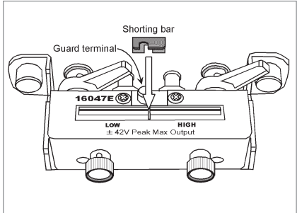
Connecting a shorting plate
