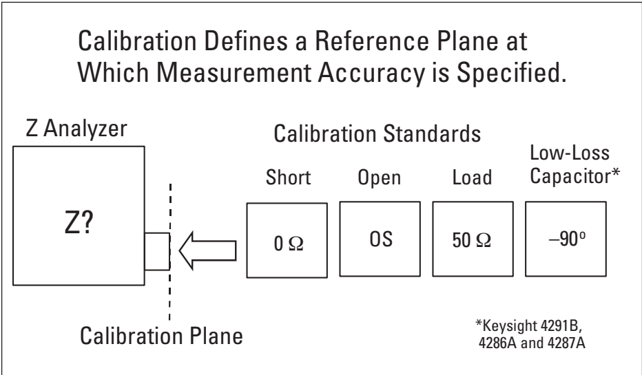
Figure 11. Calibration Plane
