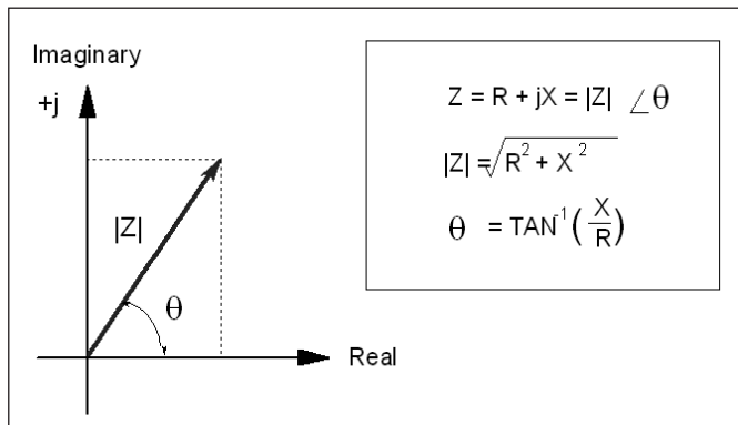
Figure 2. Impedance Vector
