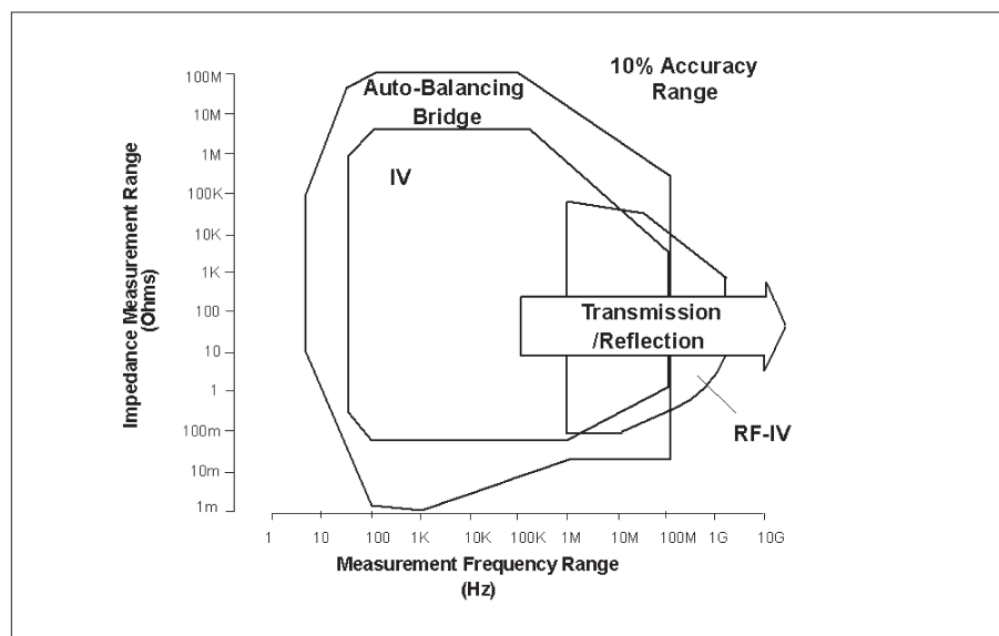
Figure 1. Accuracy Profile
