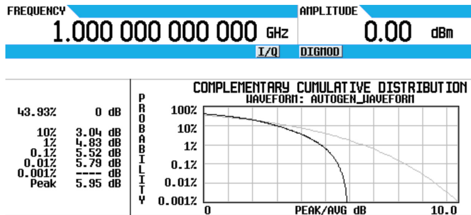
Figure 2-4. CCDF plot from waveform utility of Keysight's N5182B signal generator
