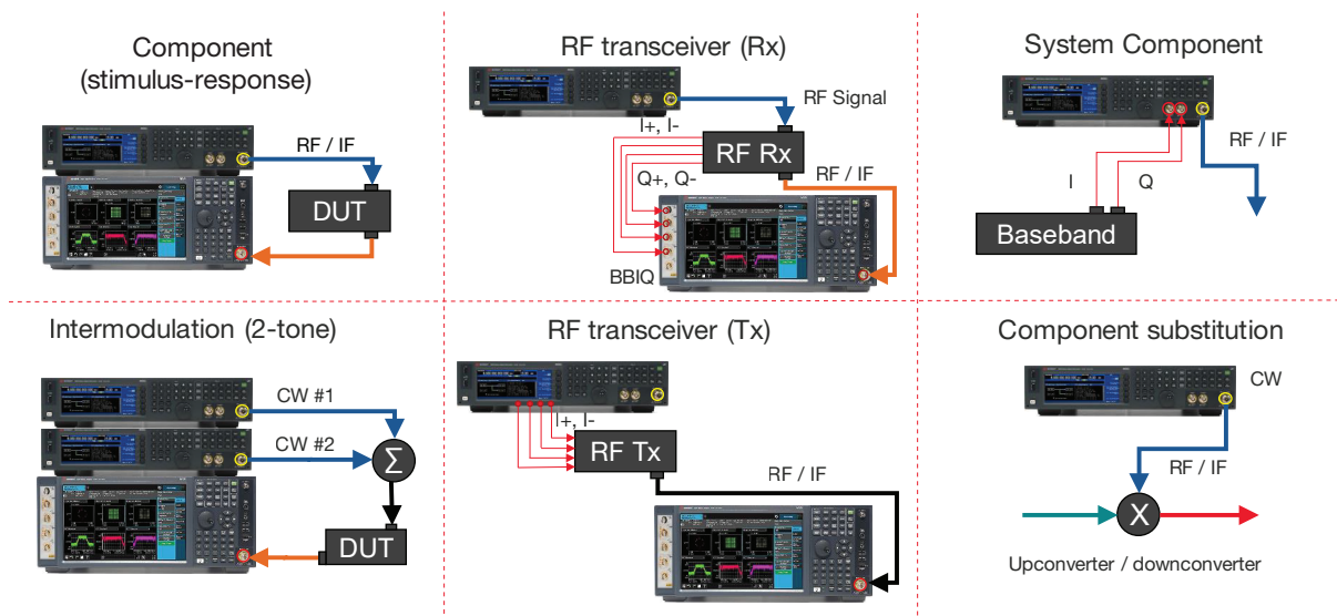
Figure 1-1. Signal generator use cases for component characteristic tests or a system component
