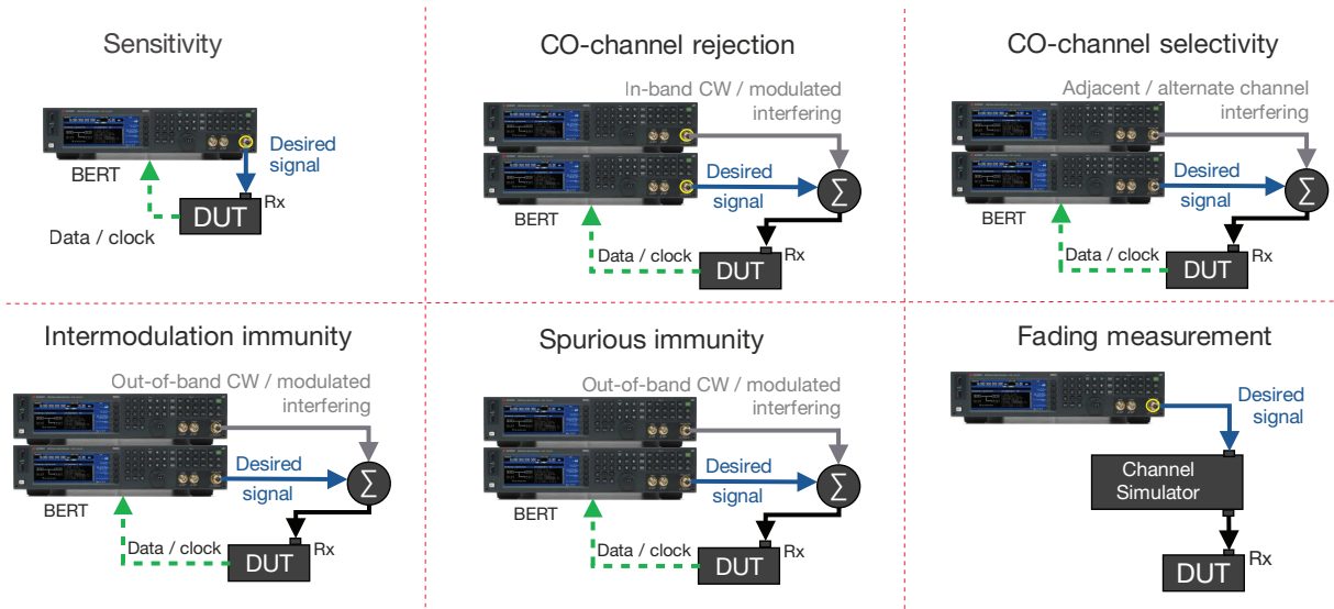
Figure 1-2. Signal generator use case for receiver sensitivity tests
