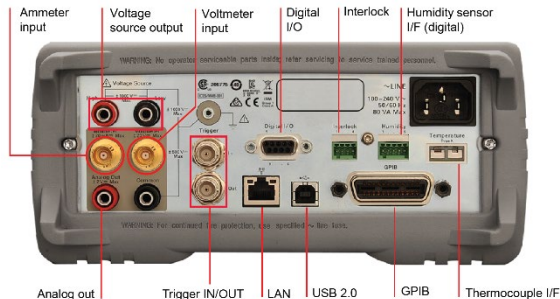
B2985A, B2987A Electrometer/High Resistance Meter
