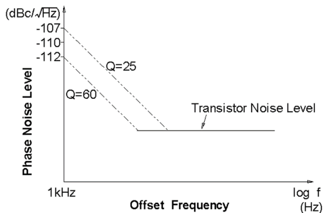
Figure 8. Improved phase noise resulted from using a high Q inductor, selected by measuring the Q at 30MHz with a 4285A Precision LCR Meter.
