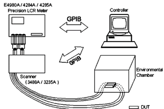
Figure 3. Accurate measurements with the test fixture extended from the LCR meter are provided with the cable extension function
