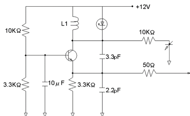
Figure 6. Part of VCO circuit used in a 20 Hz to 30 MHz synthesizer.
