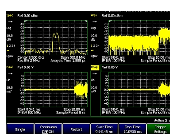
IQ data captured in FieldFox I/Q analyzer mode
