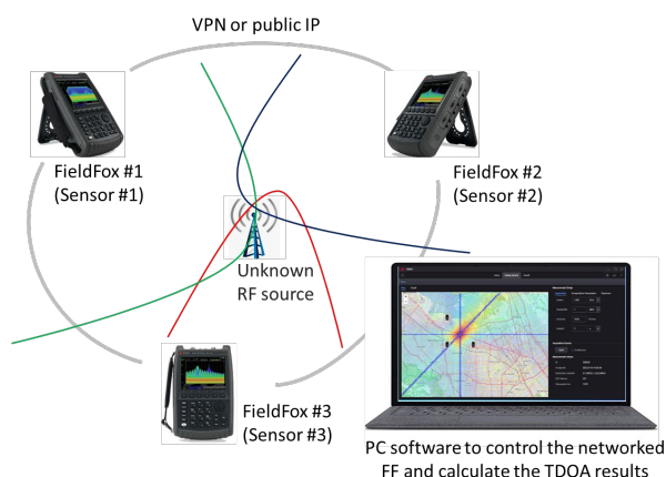
TDOA solution using three networked FieldFox analyzers and PC software KSMS
