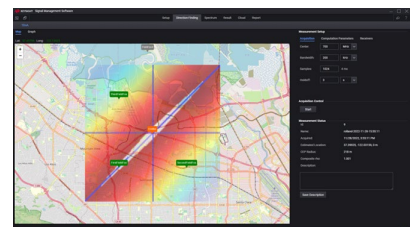
TDOA by three FieldFox analyzers
