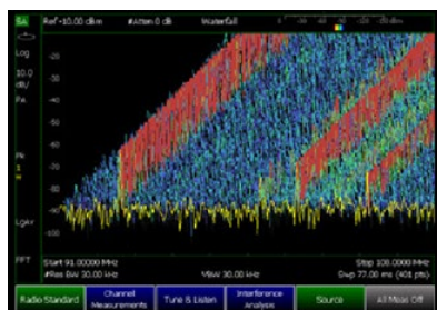
Waterfall display makes interference hunting easier
