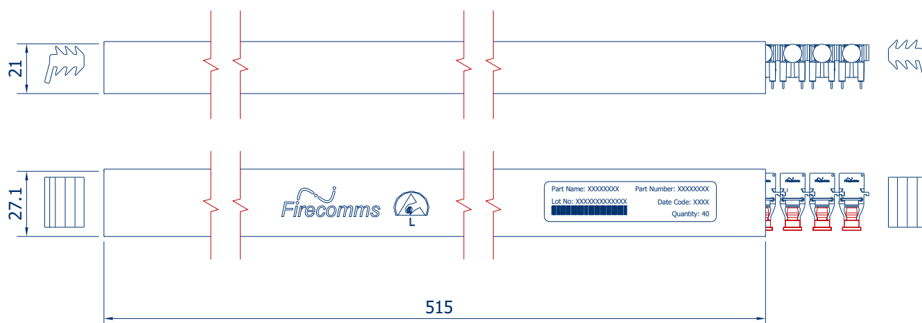
FIGURE 7 Packing tube for Firecomms RedLink® tilted connectors
