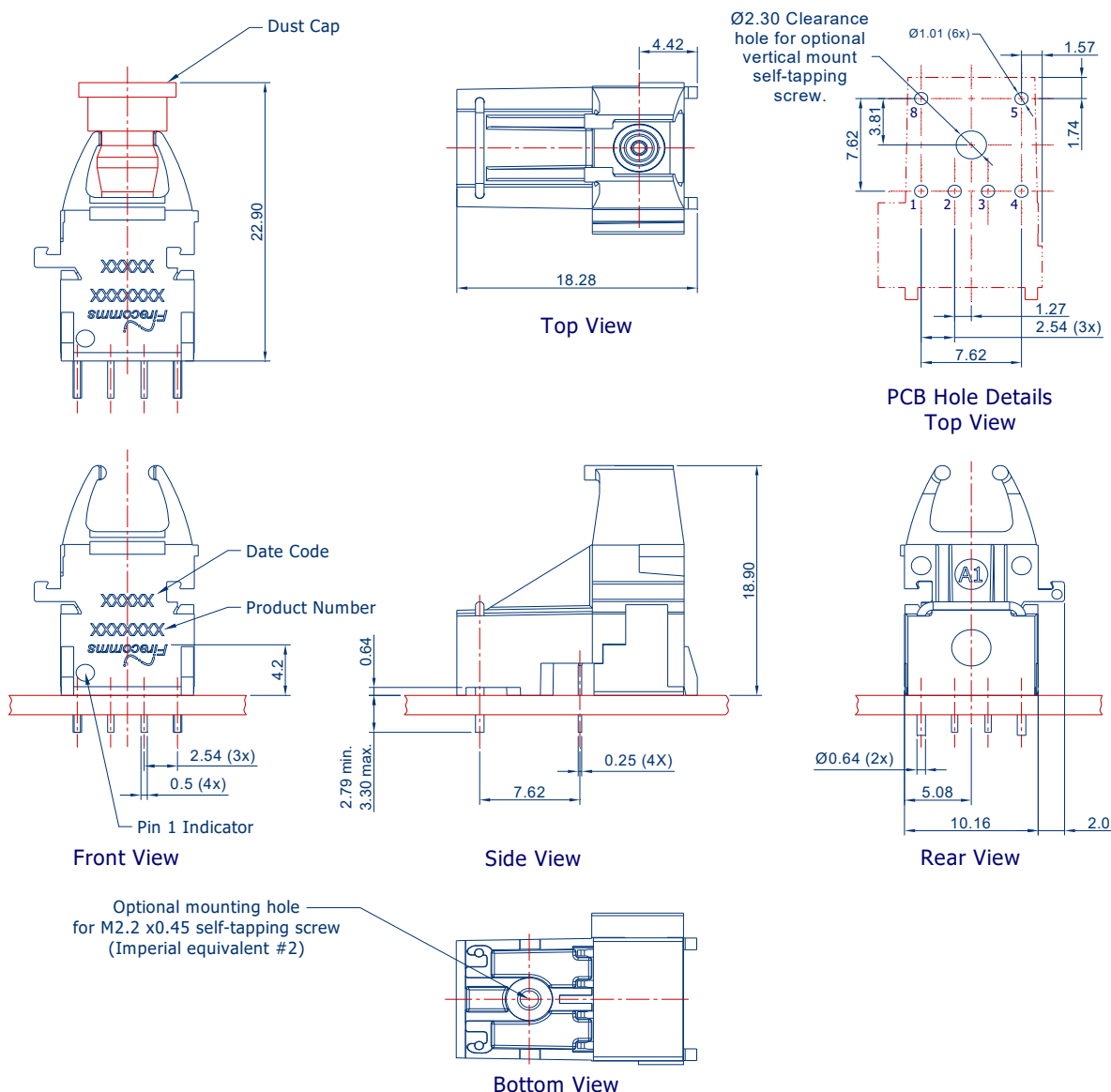
FIGURE 4 Mechanical dimensions of RedLink® vertical connectors and PCB footprint, which is a top view General dimensional tolerance is \pm 0.2 mm
