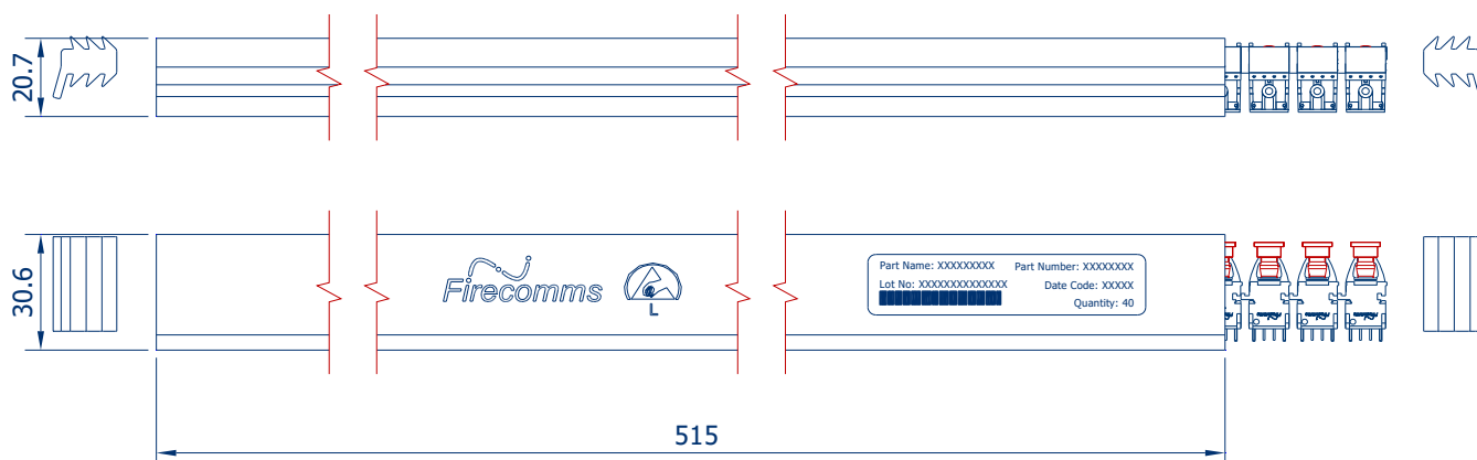
FIGURE 5 Packing tube for Firecomms RedLink® vertical connectors
