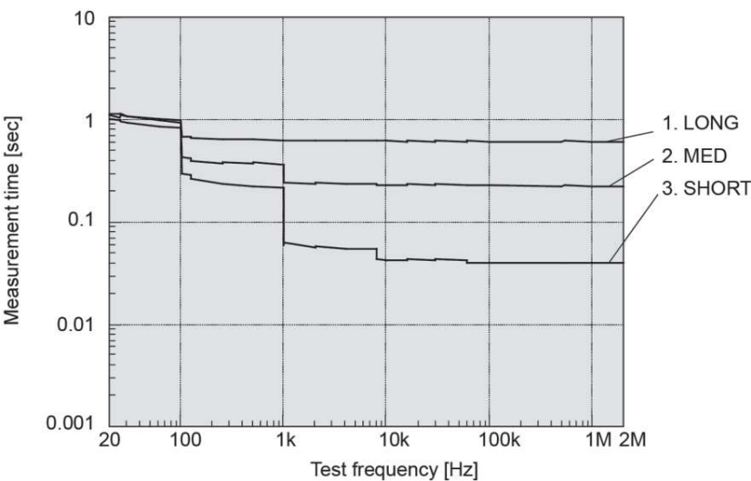
Figure 10. Measurement time (E4980BL)
