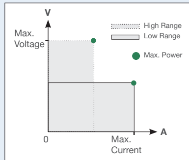
Dual-Range Operation
