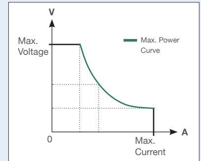
Multi-Range Operation
