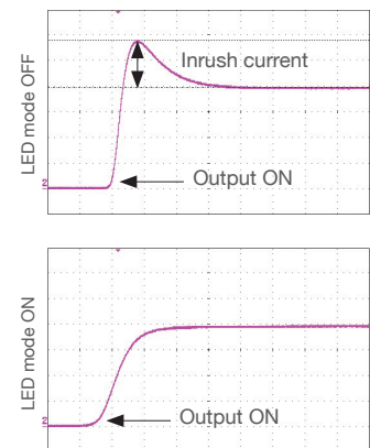
Current flow during power up with LED mode enabled
