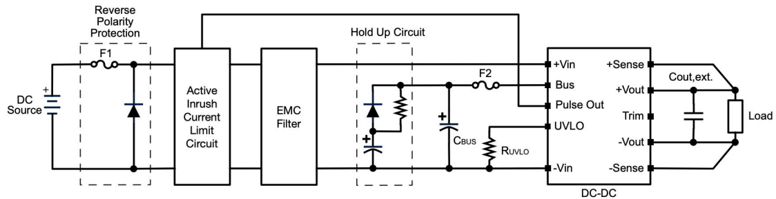
Typical Connection
