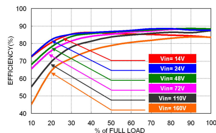
RCD20-72D15U Efficiency vs. Output Load
