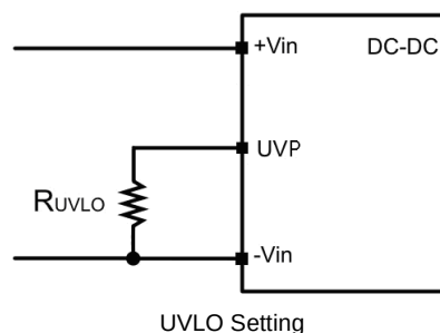
UVLO Setting
