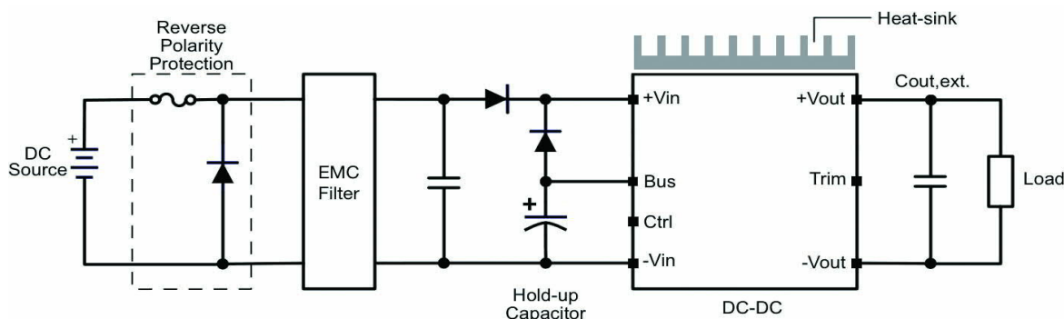
Typical Connection
