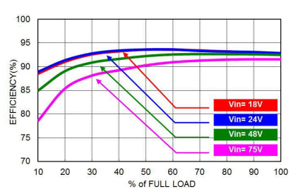
HAE300-48S28W Efficiency vs. Output Load
