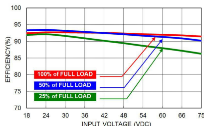
HAE300-48S28W Efficiency vs. Input Voltage
