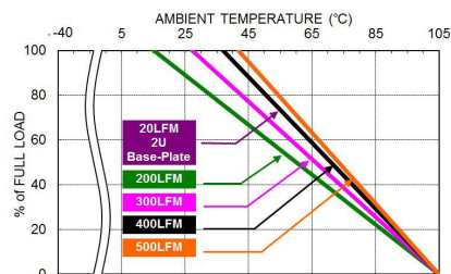
HAE300-48S28W Derating Curve (See Thermal Considerations)
