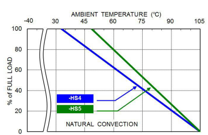
HAE300-48S28W Derating Curve with Heat-sink (See Thermal Considerations)
