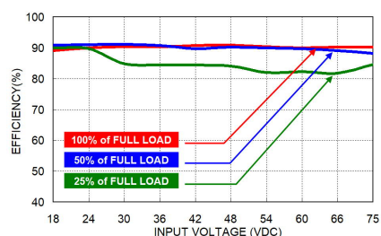
QBE100-48S05W Efficiency vs. Input Voltage
