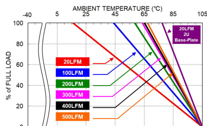
QBE100-48S05W Derating Curve
