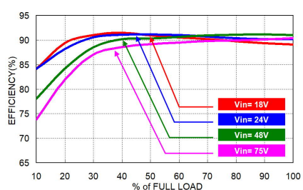
QBE100-48S05W Efficiency vs. Output Load
