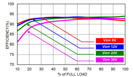
FED100-24S15W Efficiency vs. Output Load
