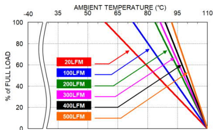
FED100-24S15W Derating Curve (Mount on 5"x3" evaluation board)
