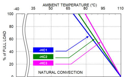
FED100-24S15W Derating Curve With Heat-sink (Mount on 5"x3" evaluation board)
