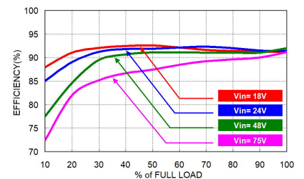
LCD50-48S12W Efficiency vs. Output Load
