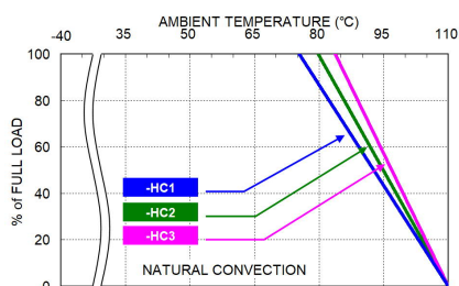
LCD50-48S12W Derating Curve With Heat-sink (Mount on 3"x3" Evaluation board)
