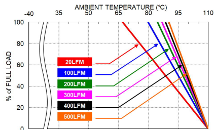
LCD50-48S12W Derating Curve (Mount on 3"x3" Evaluation board)
