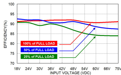
LCD50-48S12W Efficiency vs. Input Voltage
