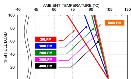
FED40-48S05W Derating Curve
