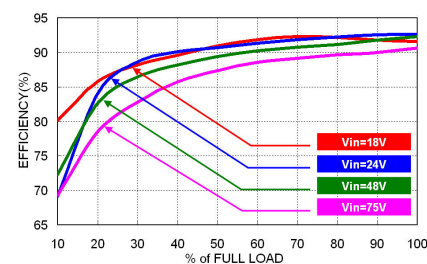
FED40-48S05W Efficiency vs. Output Load
