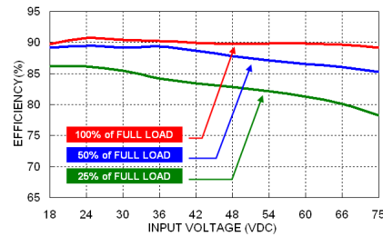
RCD20-48S05W Efficiency vs. Input Voltage
