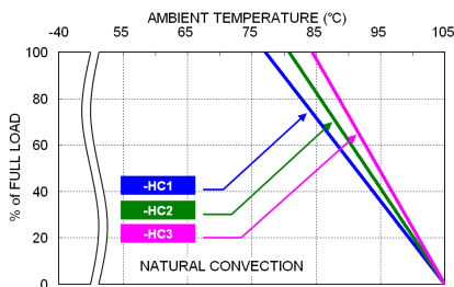
RCD20-48S05W Derating Curve With Heat-sink
