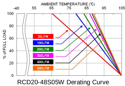
RCD20-48S05W Derating Curve
