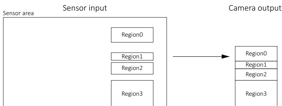
Figure 11: Vertical mode - sensor input vs. camera output
