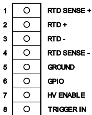
Figure 7-2 RTD/GPIO/HVEnable/Trigger connections
