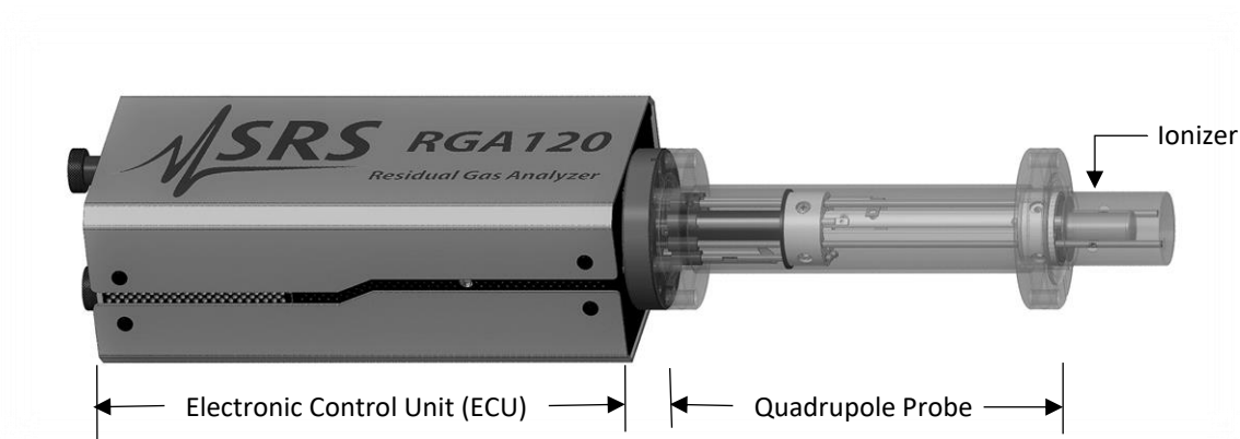
Figure 2-1 Quadrupole Head Components
