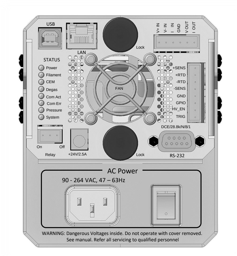
Figure 4-3 ECU Rear Panel with built in power supply module (Option 2)
