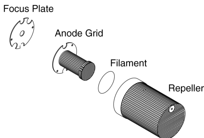
Figure 3-3 Ionizer Components
