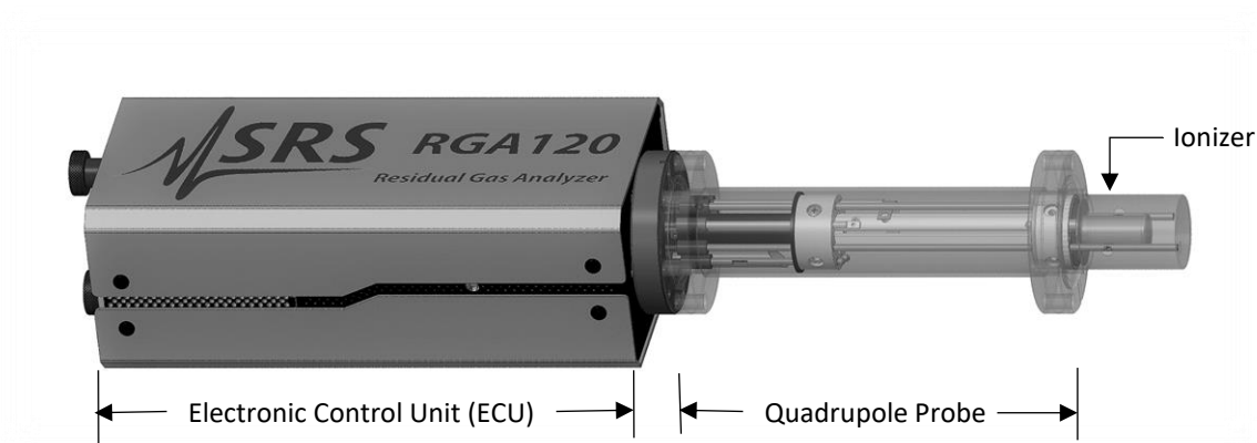
Figure 4-1 Quadrupole Head Components
