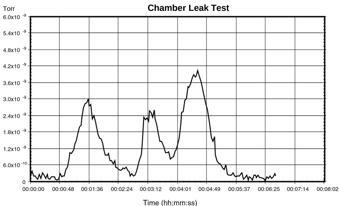
Figure 6: Helium Leak Test Data
