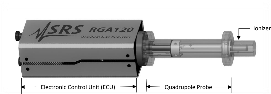
Figure 3-1 Quadrupole Head Components
