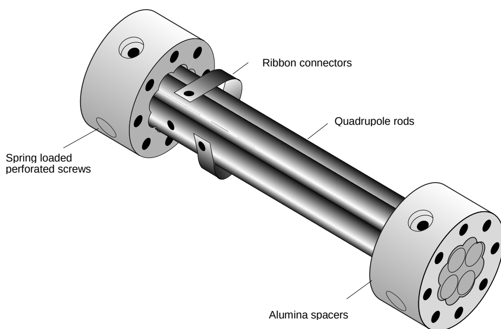
Figure 3-5 Quadrupole Mass Filter Components
