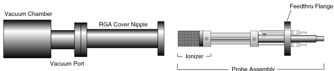
Figure 10-1 Probe Removal for Ionizer Replacement
