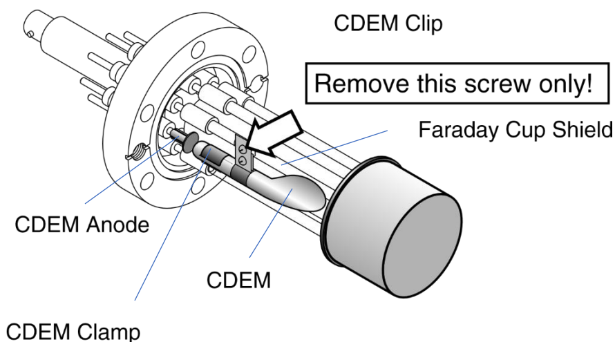
Figure 10-4 CDEM Replacement
