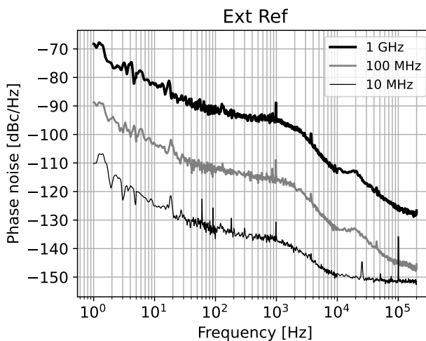
Figure 2: The phase curves (shown here at 10 MHz, 100 MHz, and 1 GHz) may be scaled by 20 dB/decade to estimate the phase noise at other frequencies.
