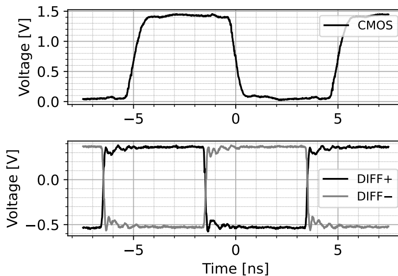
Figure 4: The trace shows a 100 MHz clock output. The 20% to 80% rise times are 75 ps and 0.6 ns, respectively, for the differential and CMOS outputs.
